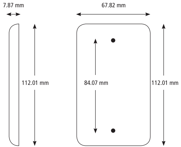
Single-gang box mounting
